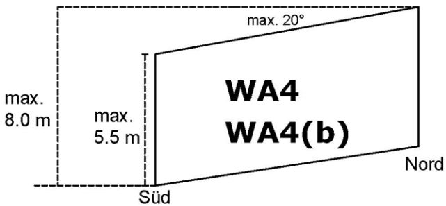
Pulldach 1
