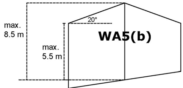
Satteldach
